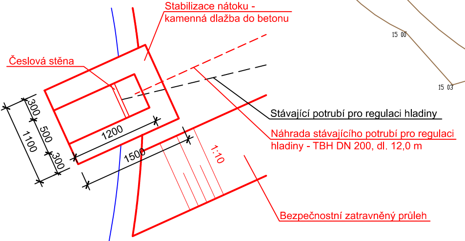
Detail 2 M 1:50
